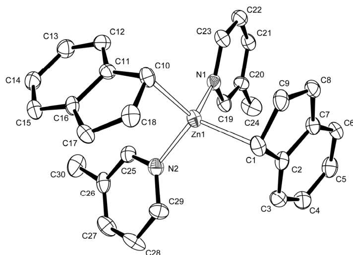
Figure 13-1. Molecular structure of ( R,R )- \alpha -17 displaying the crystallographic numbering scheme. Displacement ellipsoids are drawn at the 50% probability level and all H atoms have been omitted for clarity.
