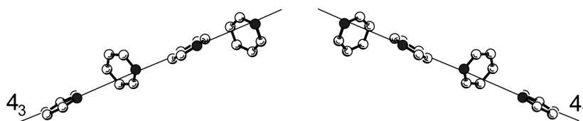
Figure 9-3. Distribution of pyridine molecules along a 4_3 - and a 4_1 -axis, respectively.
