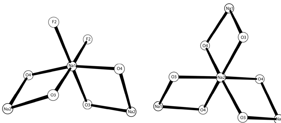
Figure 7-2. Illustration of the chiral environments around Na1 and Na2, respectively.
