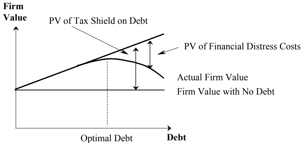
Figure 5 Optimal Leverage
