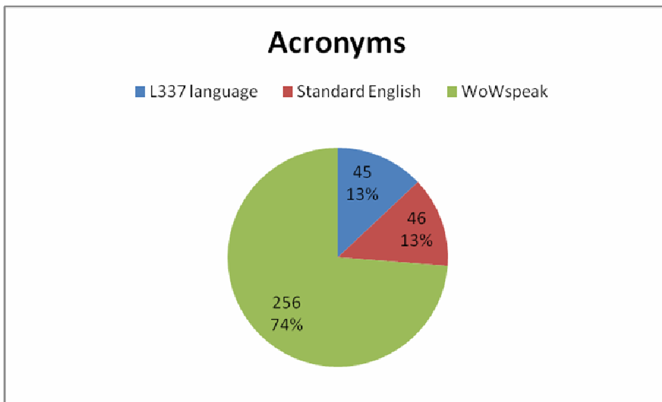
Figure 2: Percentage (out of 347) of the possible uses of the acronyms found.
