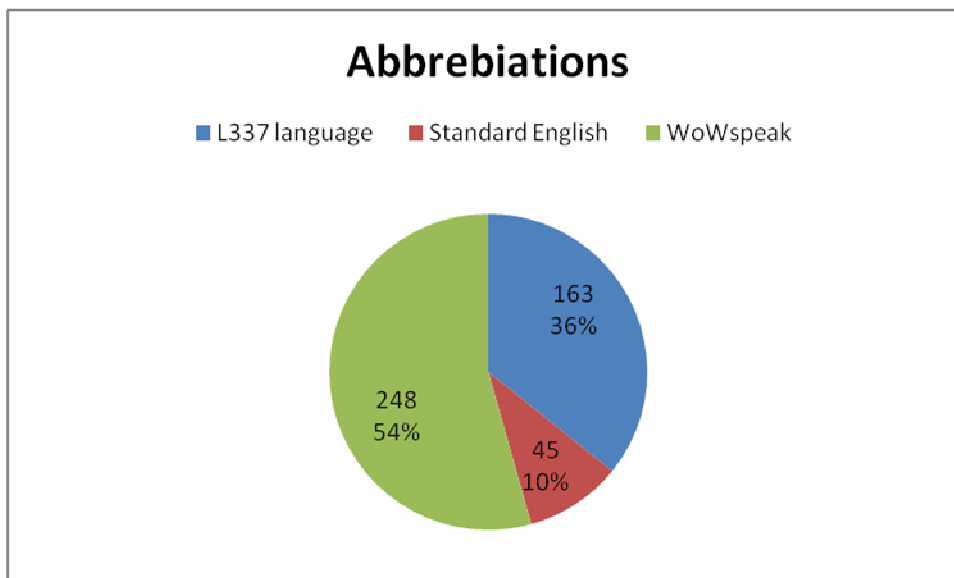
Figure 1: Percentage (out of 456) of the possible uses of the abbreviations found.
