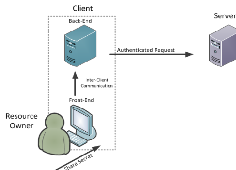
Figure 4-8 3-legged web application
