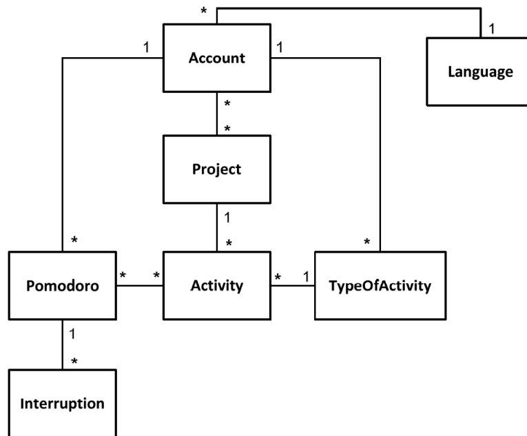
5-1 Pomodoro domain model
