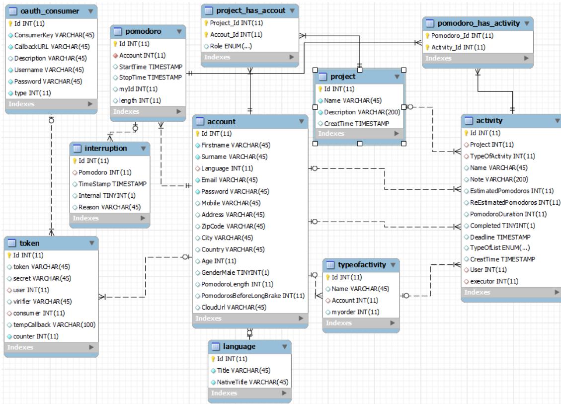
Figure 5-2 Pomodoro project E-R diagram
