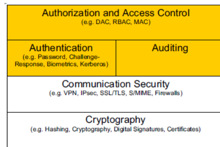
Figure 4-6 Level of security mechanisms [50]
