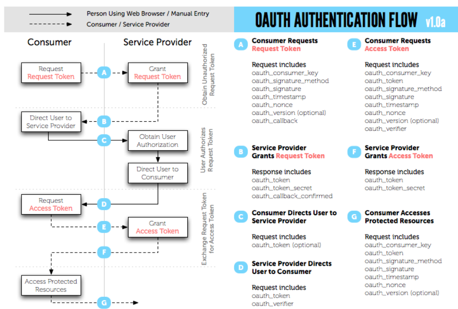
Figure 4-10 OAuth work flow [53]
