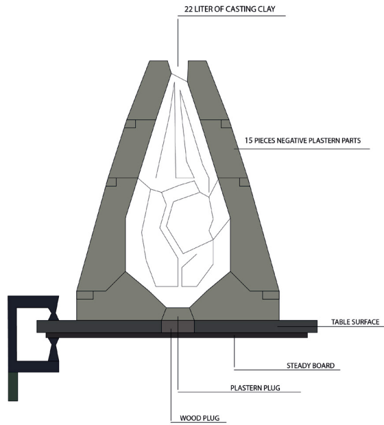
CASTING SYSTEM
