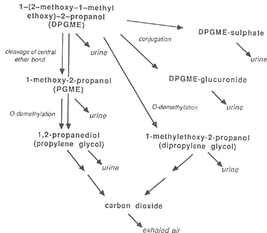
Figure 3. The metabolism of dipropylene glycol methyl ether.
