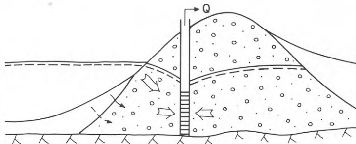
Figur 8.3. Inducerad infiltration.
