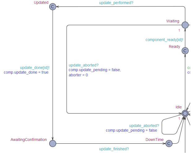
Fig. 11. A cutout of the PassiveComponent automata from UPPAAL that simulates the components update mechanism.
