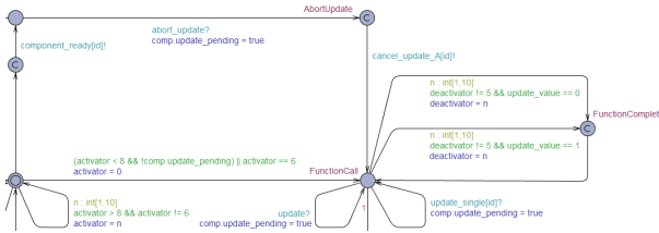
Fig. 9. A cutout of the ActiveComponent automata from UPPAAL that simulates the components abort mechanism as well as its working behaviour.
