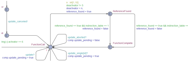
Fig. 10. A cutout of the PassiveComponent automata from UPPAAL that simulates the component being active.
