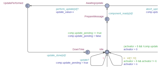
Fig. 7. A cutout of the ActiveComponent automata from UPPAAL that simulates the components update mechanism.
