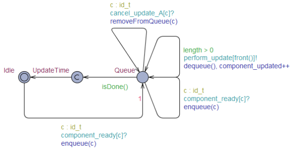
Fig. 8. ActiveDSU automata from UPPAAL.
