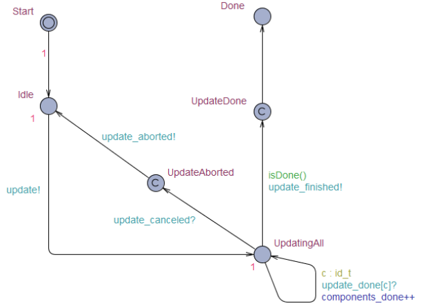
Fig. 6. Manager automata from UPPAAL.
