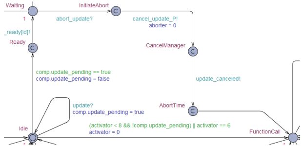
Fig. 12. A cutout of the PassiveComponent automata from UPPAAL that simulates the components abort mechanism.
