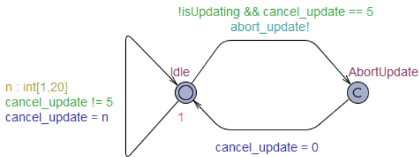
Fig. 5. InterruptHandler automata from UPPAAL.
