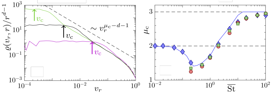
Figure 4.2: Statistical model simulations for d = 2 , Ku = 1 Left: \rho(v_r, r)/r^{d-1} evaluated for small r , \overline{St} = 1 and \theta = 10^{-3} , 10^{-2} and 10^{-1} as the green, black and magenta lines, respectively. The crossover scales v_c are shown as arrows. Right: Power-law exponent \mu_c as a function of \overline{St} for small \theta . Exponent for the power-law tails in v_r for fixed small r with \theta = 10^{-3} (green boxes) and \theta = 10^{-2} (red circles). Exponent for power-law tails in r for fixed small v_r with \theta = 10^{-2} (blue diamonds). Numerical data for \mu_c (solid blue line). Figures taken from paper B.
