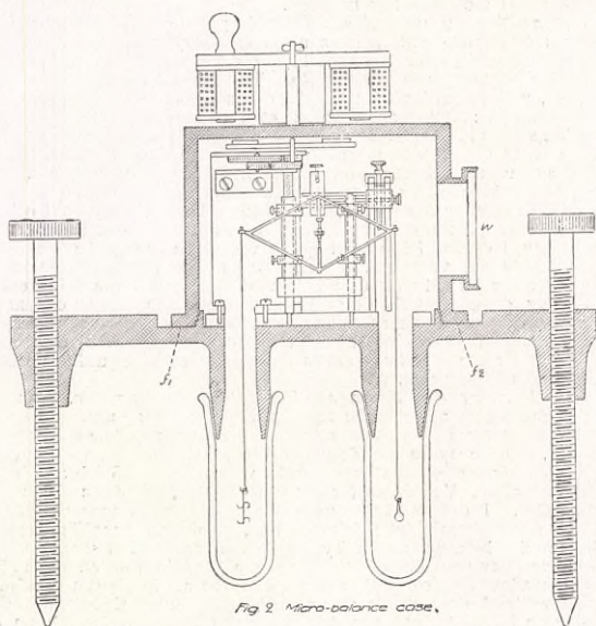
Fig 2. Micro-balance case.
