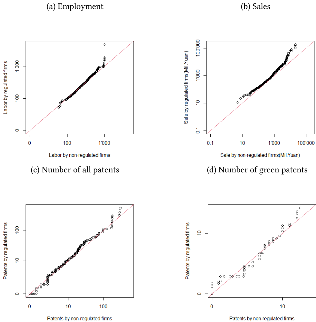
Figure 3: Quantile-quantile plots on matched sample, matching variables
