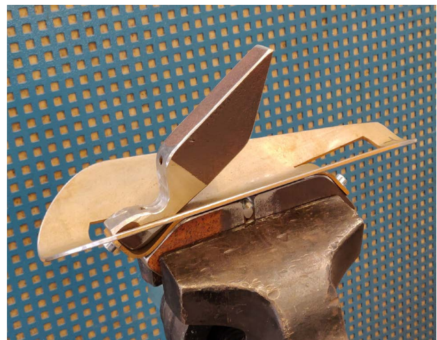
[fig.41.] special jig to bend the attachment ears
